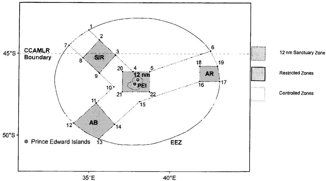
Fig. 1. The boundaries for the Prince Edward Islands Marine Protected Area.
